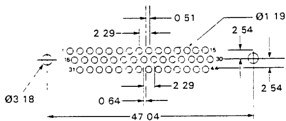
44 Contacts
