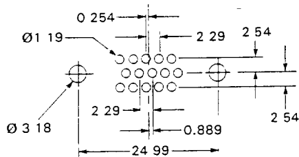
15 Contacts
