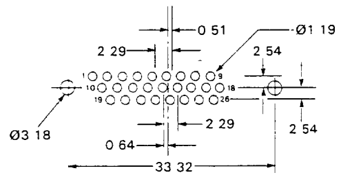
26 Contacts
