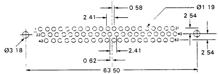
62 Contacts
