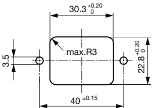
Panel cutout for rear side mounting
