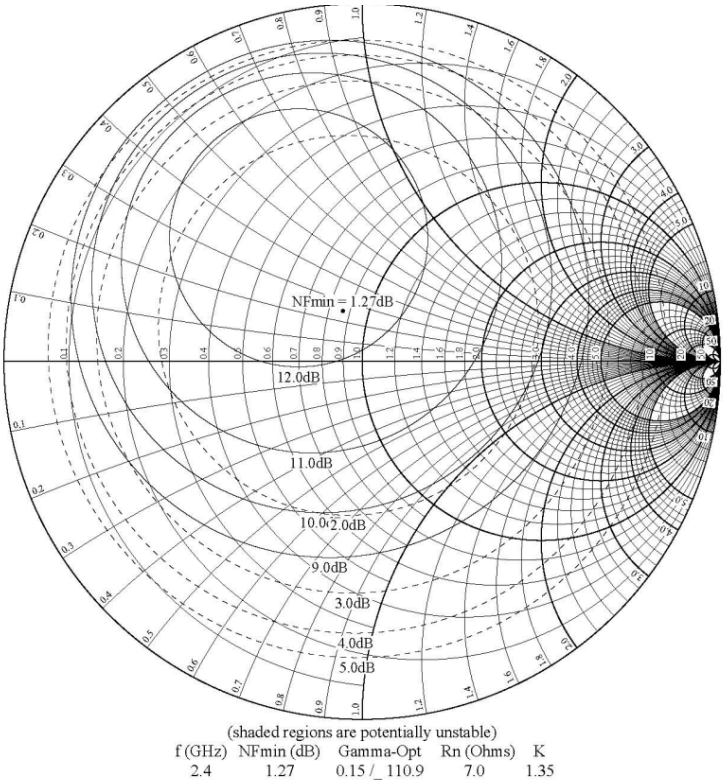
Figure 8. Constant Noise Figure and Gain Circles, 2400 MHz, Low IP3 Mode, 25 °C
