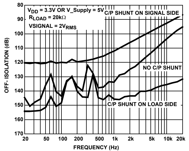
FIGURE 11. OFF-ISOLATION, 2V_{RMS} SIGNAL, 20\text{k}\Omega LOAD
