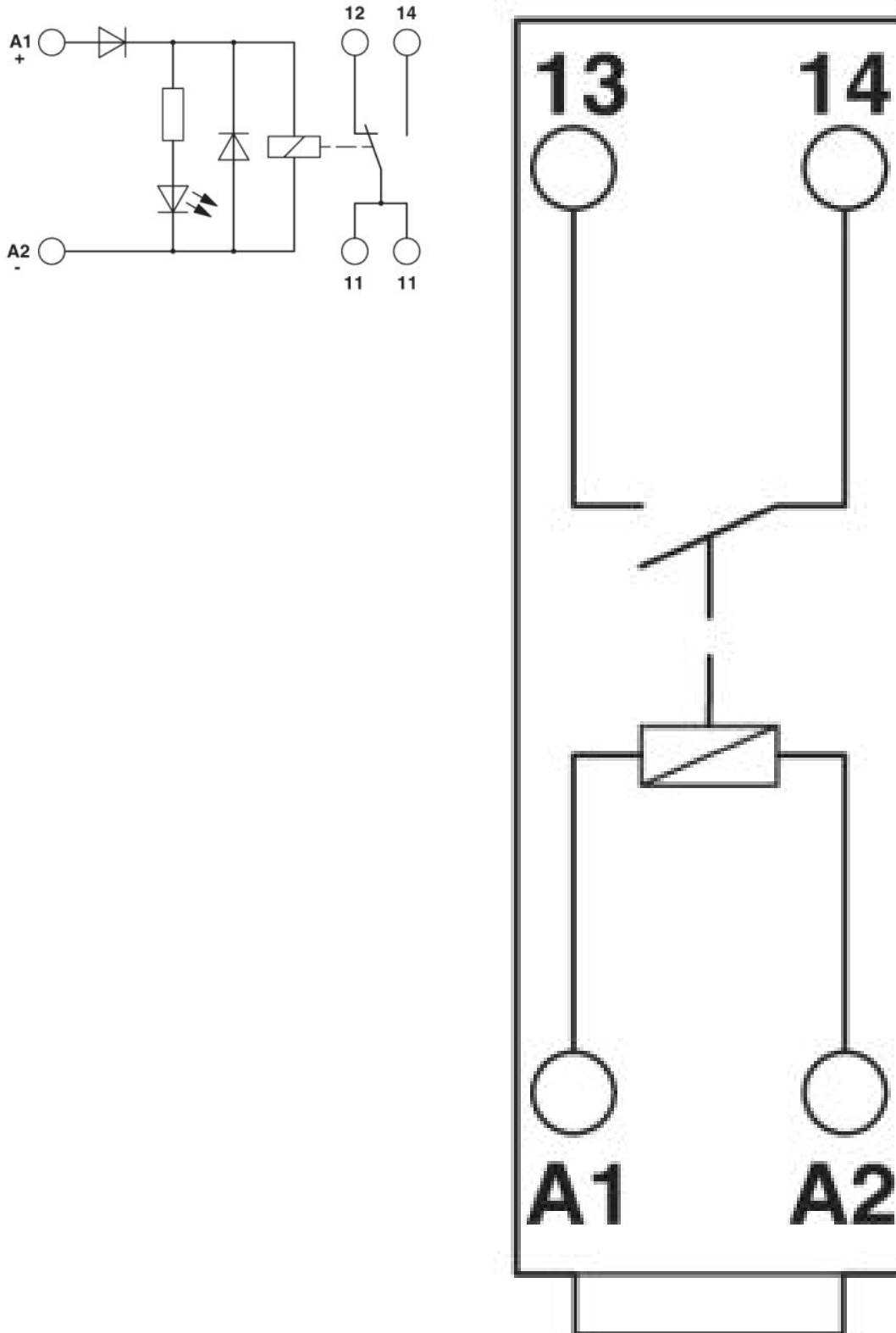
Circuit diagram
