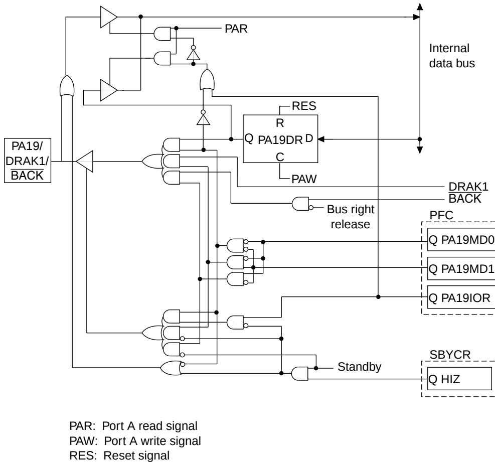
Figure B.10 PA19/DRAQ1/BACK Block Diagram
