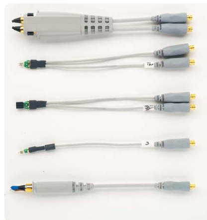
Types of InfiniiMax probe heads
