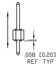
END VIEW
