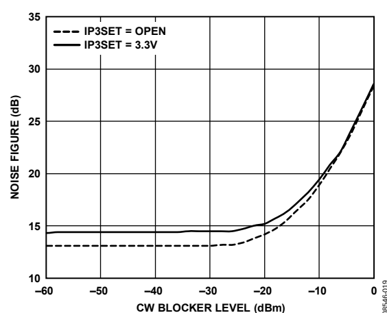
Figure 19. SSB Noise Figure vs. 5 MHz Offset Blocker Level, LO Frequency = 1055 MHz, RF Frequency = 915 MHz
