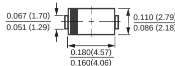
DO-214AC
