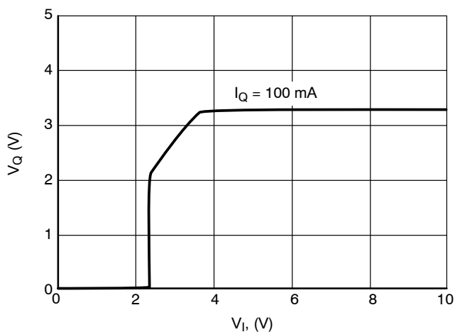
Figure 23. Output Voltage V_O vs. Input Voltage V_I
