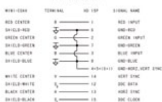
WIRING DIAGRAM
