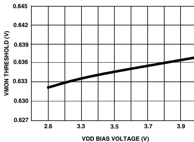
FIGURE 3. VMON THRESHOLD vs. VDD VOLTAGE
