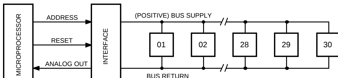
FIGURE 3 BUS INTERCONNECTION
