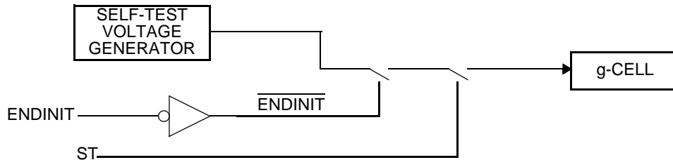
Figure 9. Self-Test Interface
