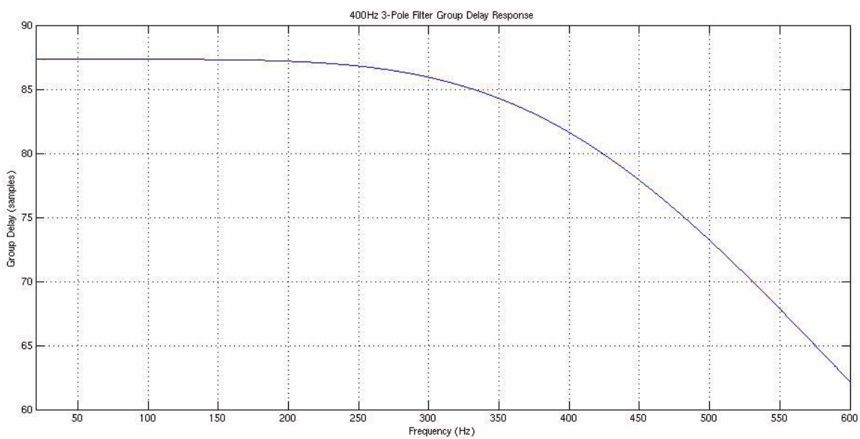
Figure 17. Low-Pass Filter Characteristics: f_C = 400 Hz, Poles = 3, t_S = 8 \mu s
