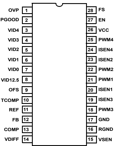
28 LEAD SOIC TOP VIEW
