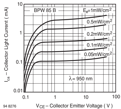
Figure 6. Collector Light Current vs. Collector Emitter Voltage
