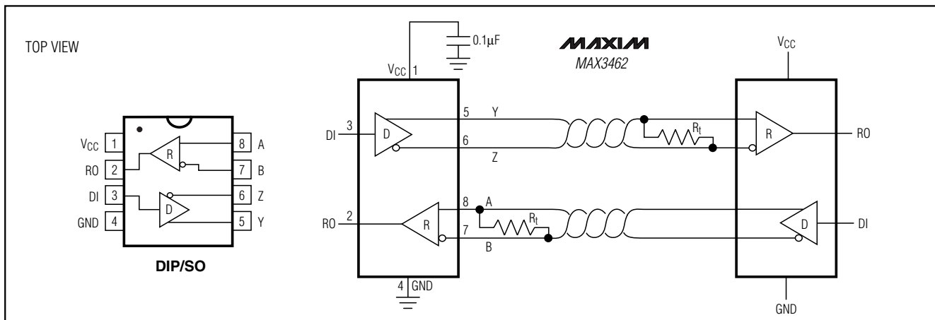
Figure 2. MAX3462 Pin Configuration and Typical Full-Duplex Operating Circuit
