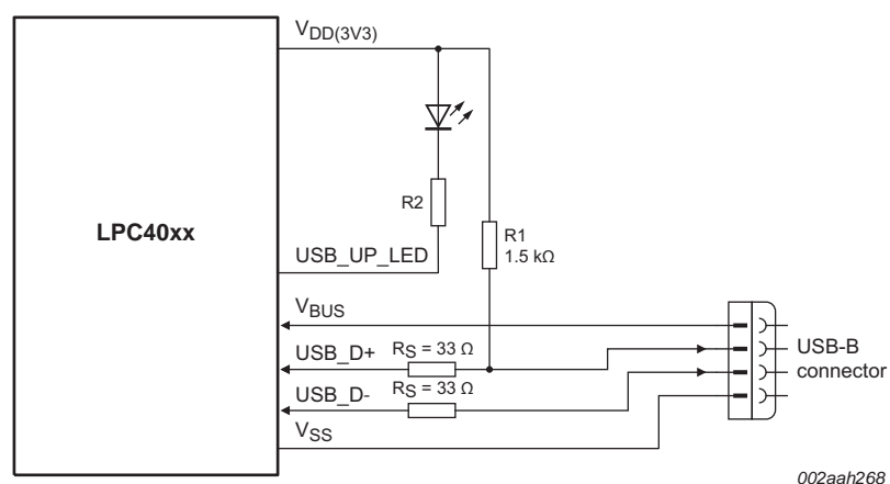
Fig 34. USB interface on a bus-powered device
