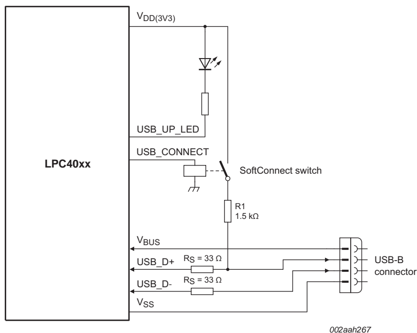
Fig 33. USB interface on a self-powered device
