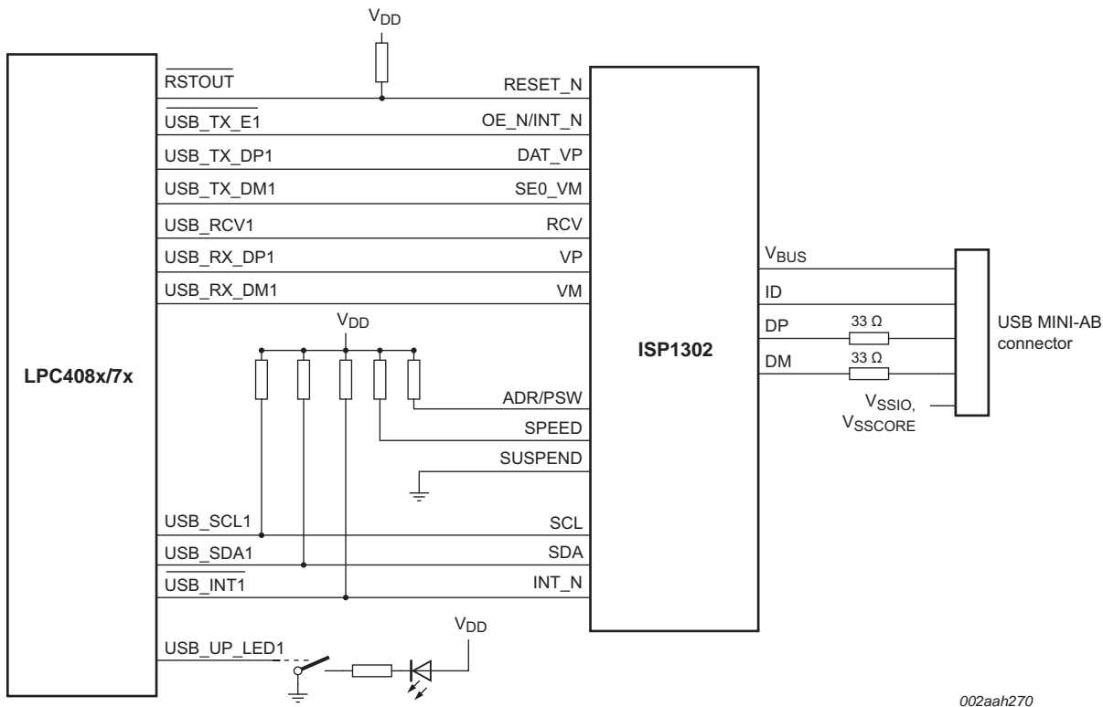
Fig 36. USB OTG port configuration: VP_VM mode
