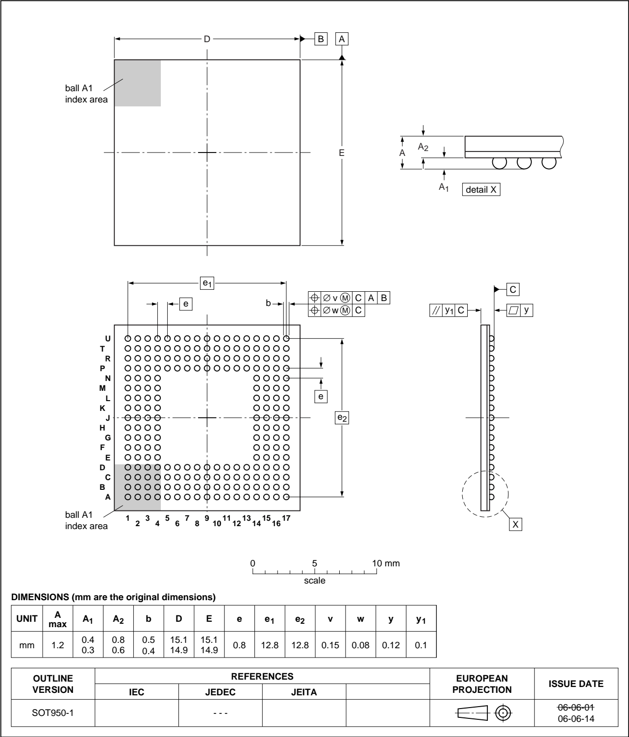
Fig 45. Package outline SOT950-1 (TFBGA208)
