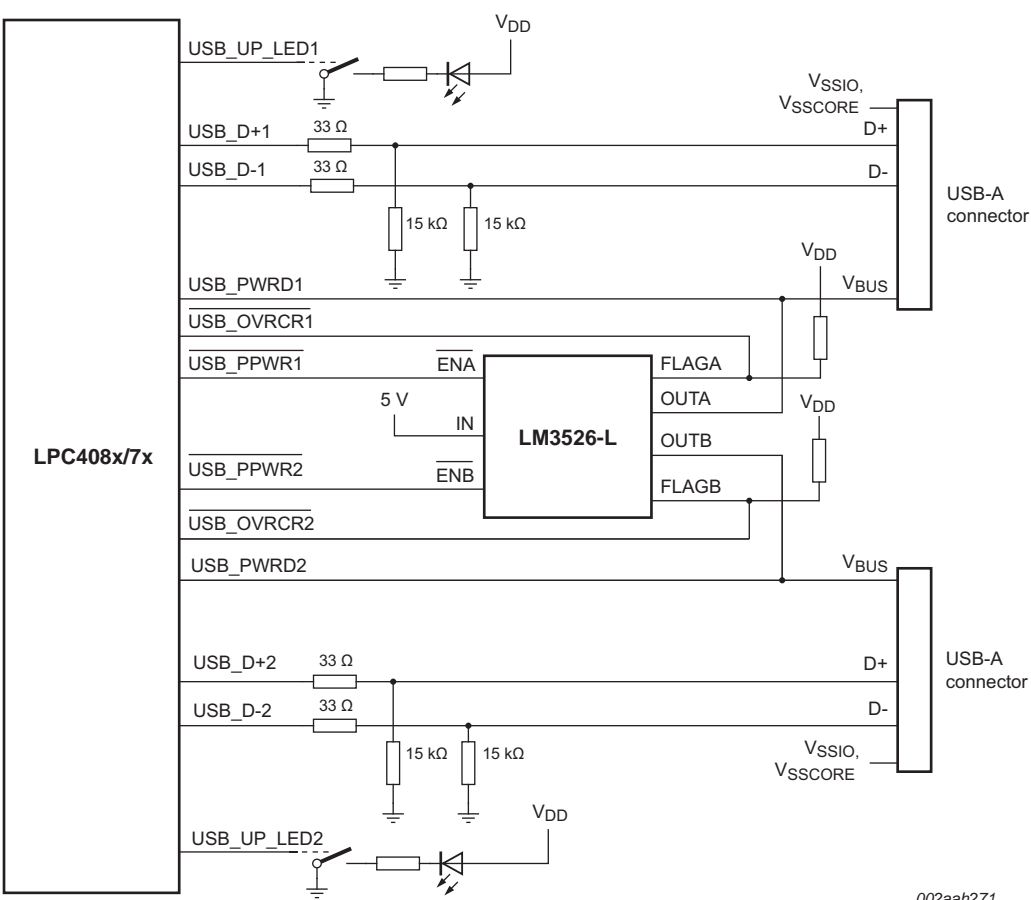
Fig 37. USB host port configuration: port 1 and port 2 as hosts
