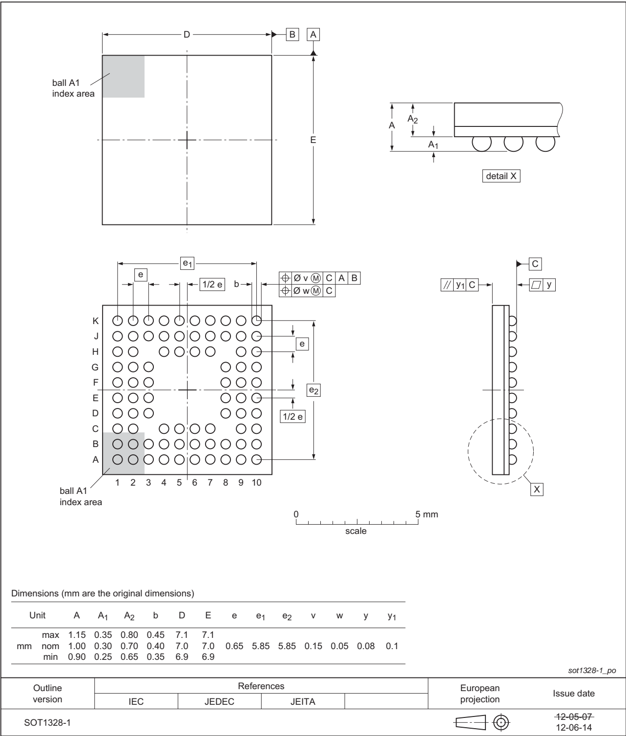
TFBGA80: plastic thin fine-pitch ball grid array package; 80 balls
