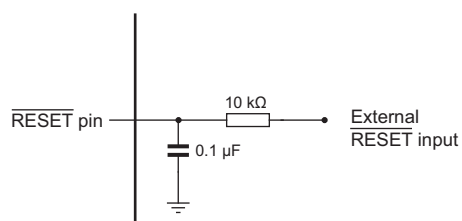
Fig 43. Reset input with RC filter
