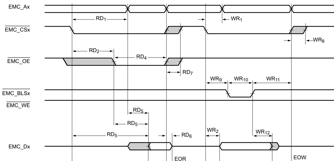
Fig 19. External static memory read/write access ( \text{PB} = 0 )
