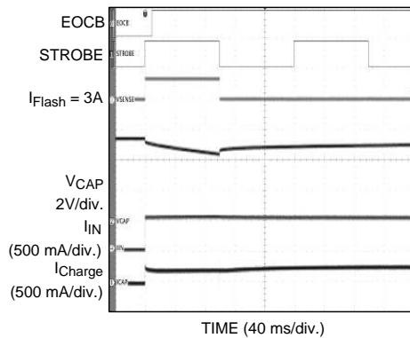
Figure 30. Edge-Sensitive Strobe
