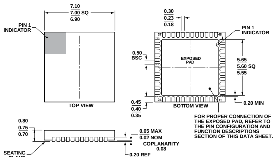
Figure 3. 48-Lead Lead Frame Chip Scale Package [LFCSP_WQ] 7 mm × 7 mm Body, Very Very Thin Quad (CP-48-13)
