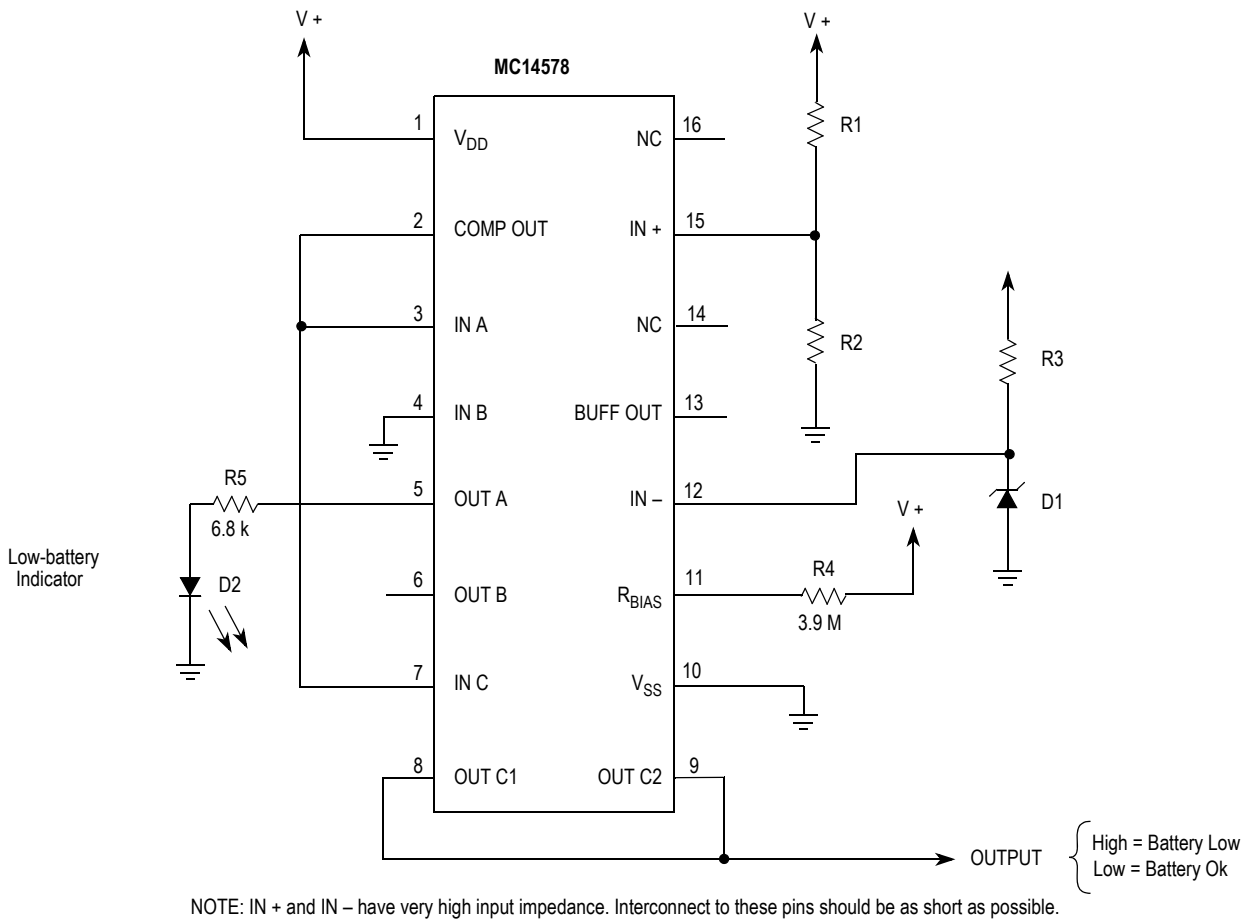
Figure 3. Low-Battery Detector
