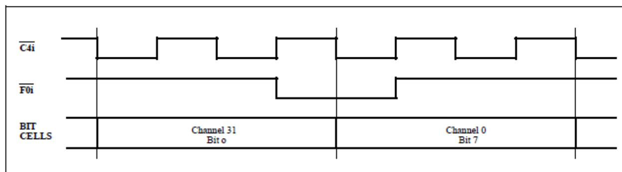
Figure 12 - Frame Alignment
