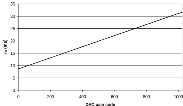
Figure 30. I_{\text{FS}} vs. DAC Gain Code
