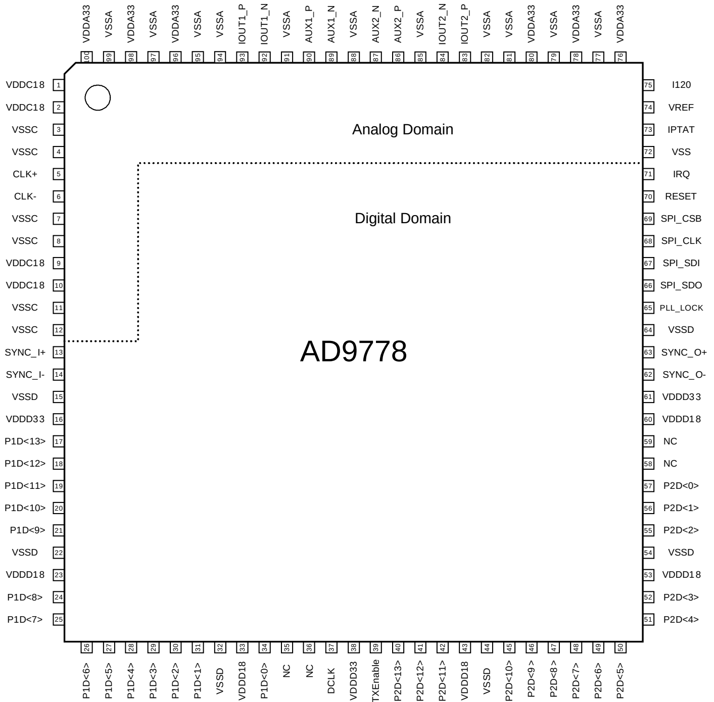
Figure 2. Pin Configuration
