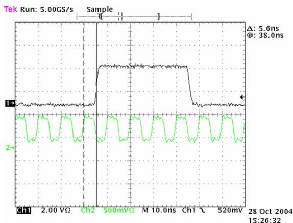
Figure 37. Delay from DACCLK to DATACLK out with CLK DATA DELAY = 000
