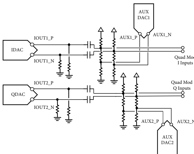
Figure 31. Typical Use of Auxiliary DACs
