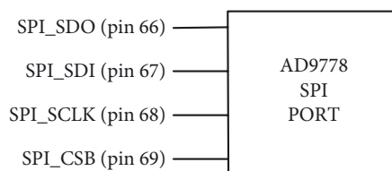
Figure 24. AD9778 SPI Port
