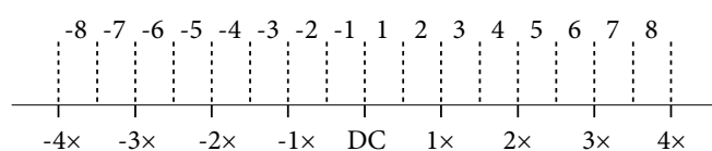
Figure 39. Nyquist Zones
