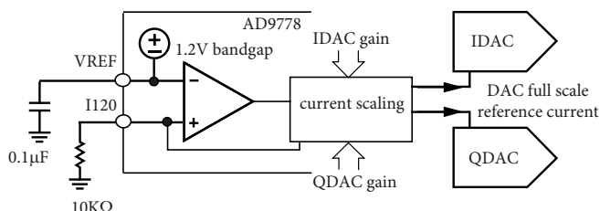
Figure 29. Reference Circuitry
