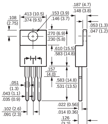
TO-220
