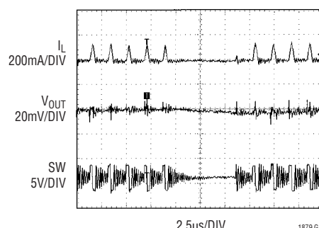
Pulse Skipping Mode Operation
