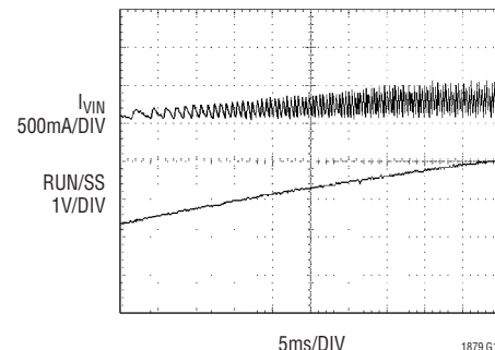
Soft-Start with Shorted Output
