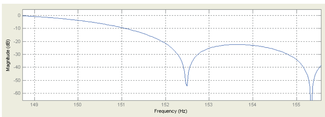
Figure 41. Frequency Response for the MBF Filter (Sharp cut off Around 150Hz)
