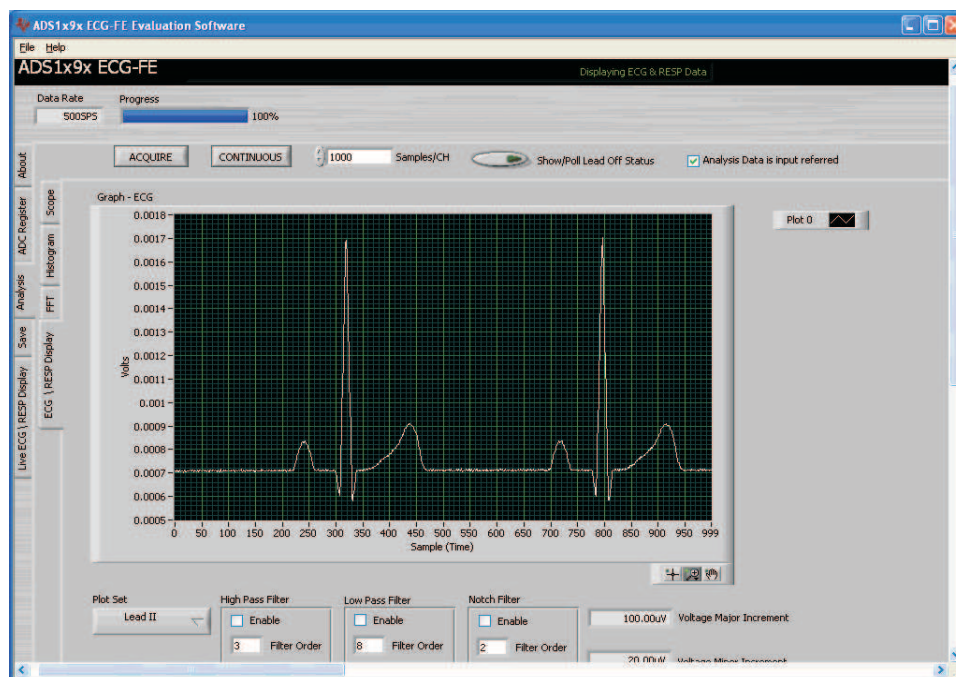
Figure 28. PC Application Analysis – ECG
