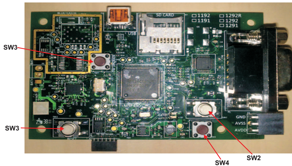
Figure 34. Switch Positions
