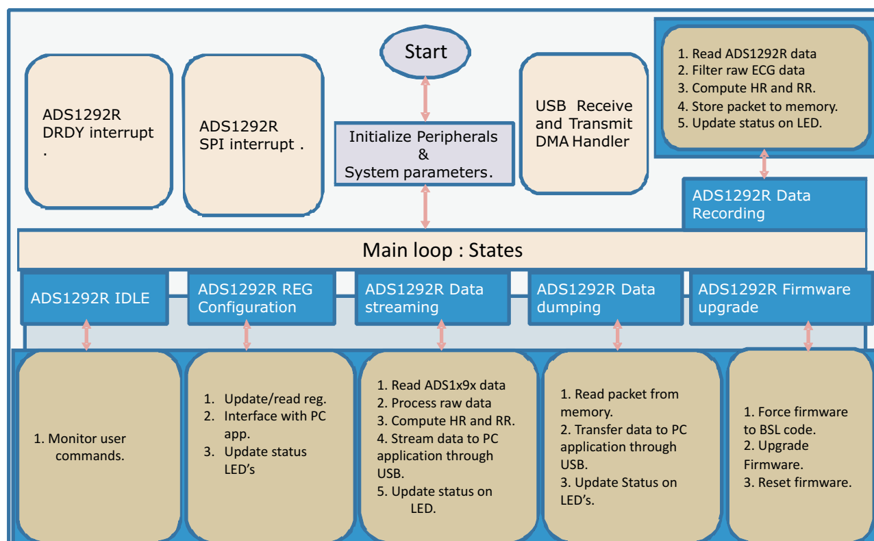
Figure 35. Firmware Architecture
