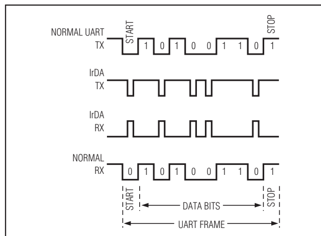
Figure 15. IrDA Timing
