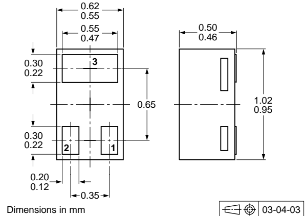
Fig 13. Package outline PDTA143XM (SOT883/SC-101)
