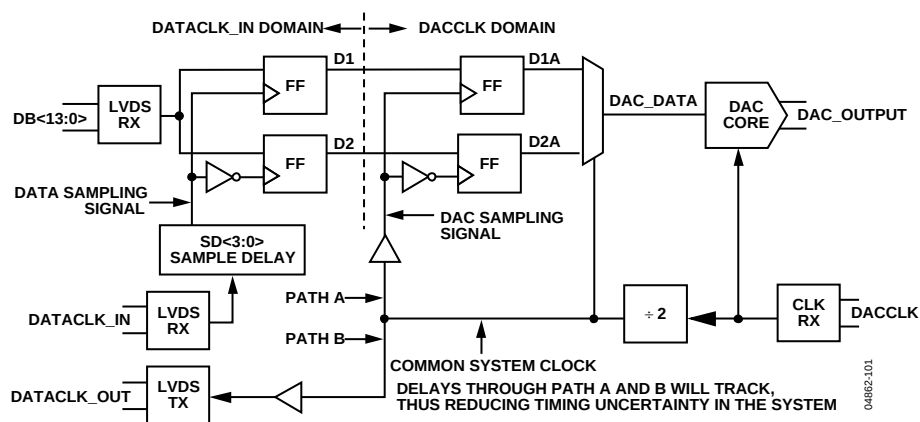
Figure 101. Simplified Internal Clock Routing
