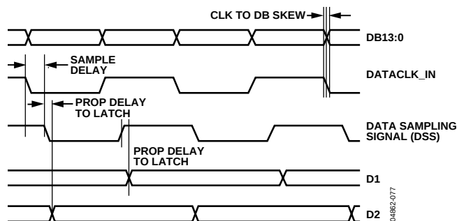
Figure 77. AD973x Internal LVDS Data Sampling Logic Timing
