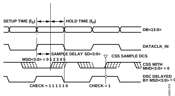
Figure 79. Hold Delay Measurement
