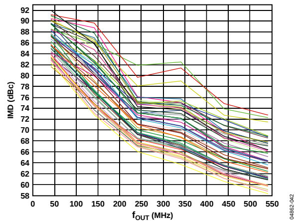
Figure 42. AD9736 IMD vs. f_{OUT} over 50 parts, 25°C, 1.2 GSPS
