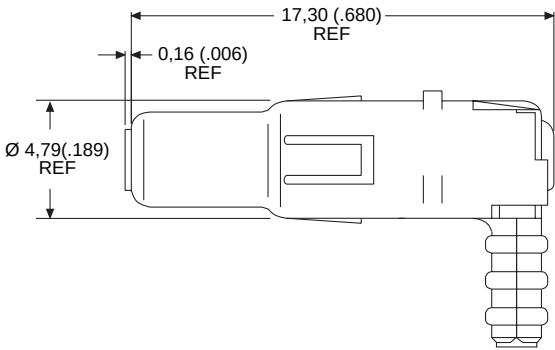
Plug
