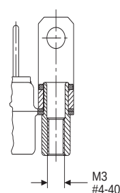
Plastic Bracket with Post (1APN/1A6N)(M3/4-40)
