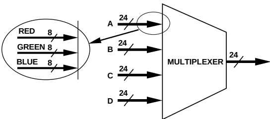
Figure 12. Multiplexed Color Inputs for the ADV7150
