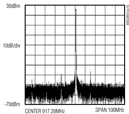
SPURIOUS LEVEL BETWEEN \pm 50MHz FROM CARRIER FREQUENCY
