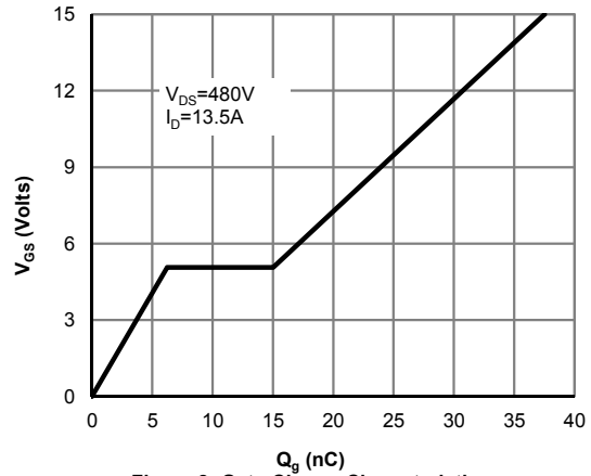
Figure 8: Gate-Charge Characteristics
