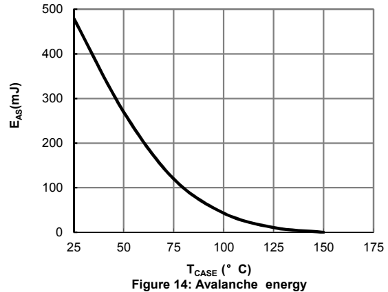
Figure 14: Avalanche energy
