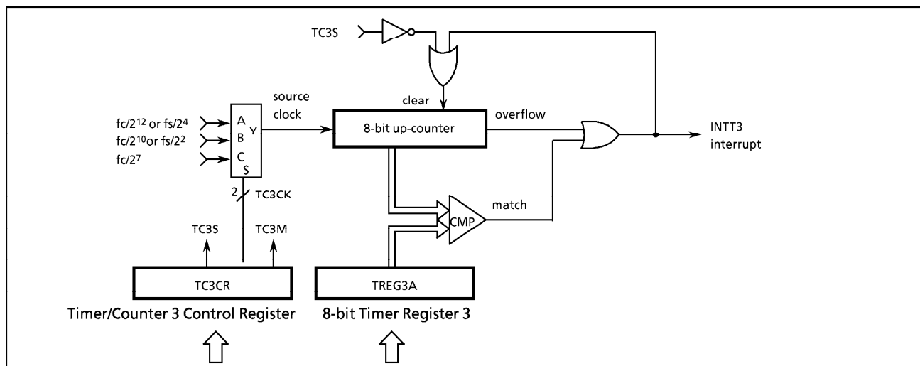
Figure 2-30. Timer/Counter 3
