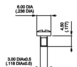
CONNECTING SCREW U03
