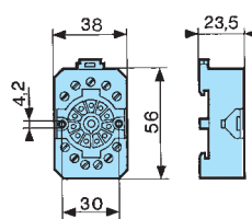
Connector socket 11-pin 25 622 077 8-pin 25 622 128
