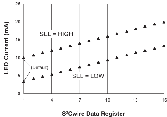
Figure 5: Programming AAT1231 LED Current with R_{\text{BALLAST}} = 30.1\Omega .
