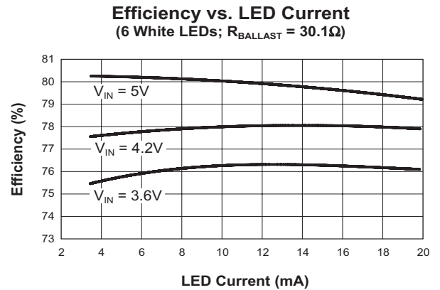
Figure 16: Six LEDs In Series Configuration.
