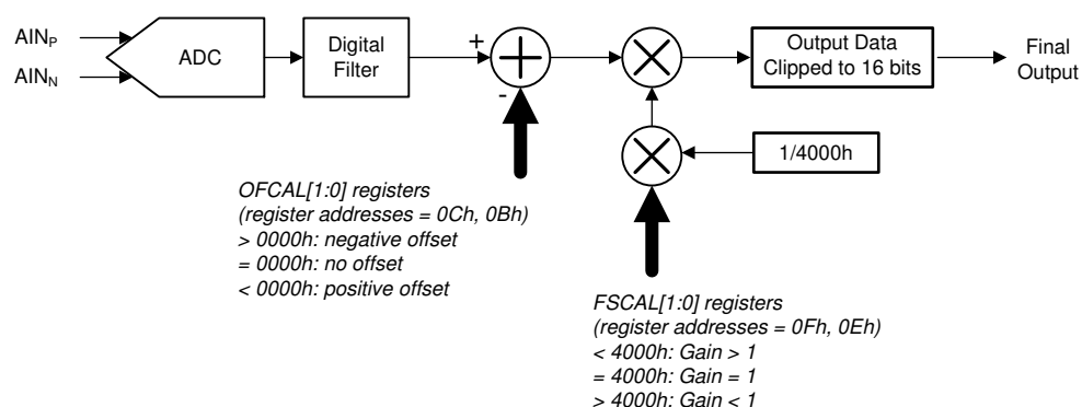
Figure 66. ADC Calibration Block Diagram
