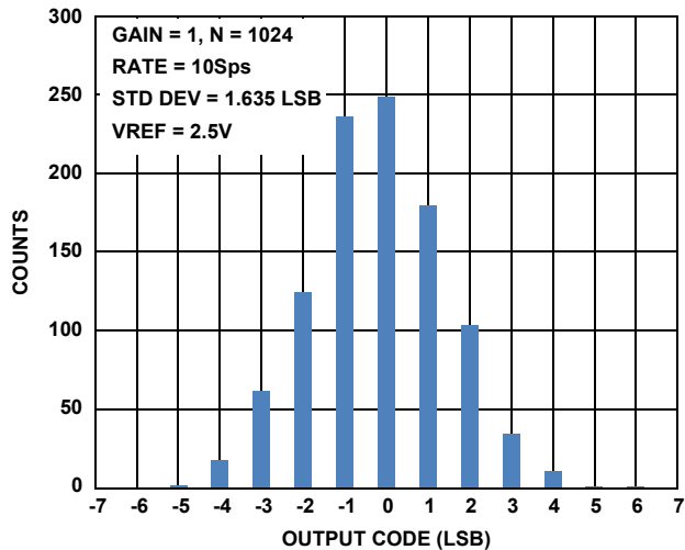
FIGURE 3. NOISE HISTOGRAM AT GAIN = 1, 10Sps
