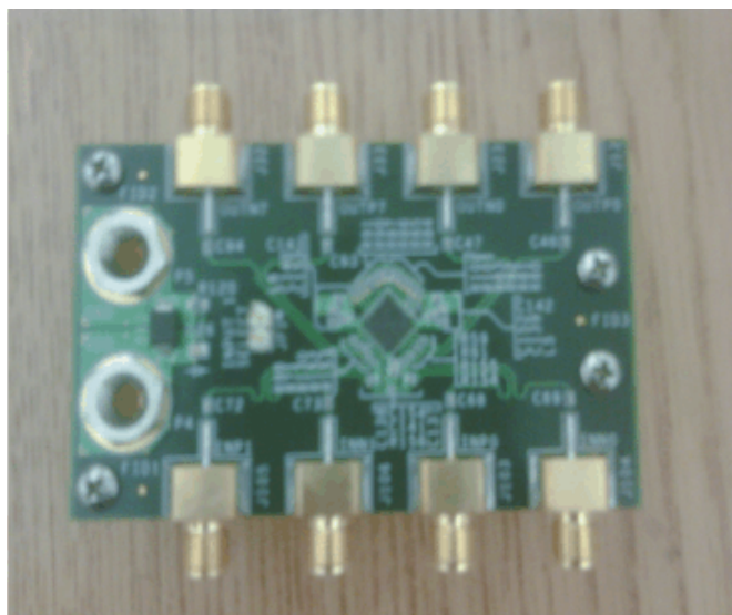
Figure 1. CDCLVP1208EVM Evaluation Board
