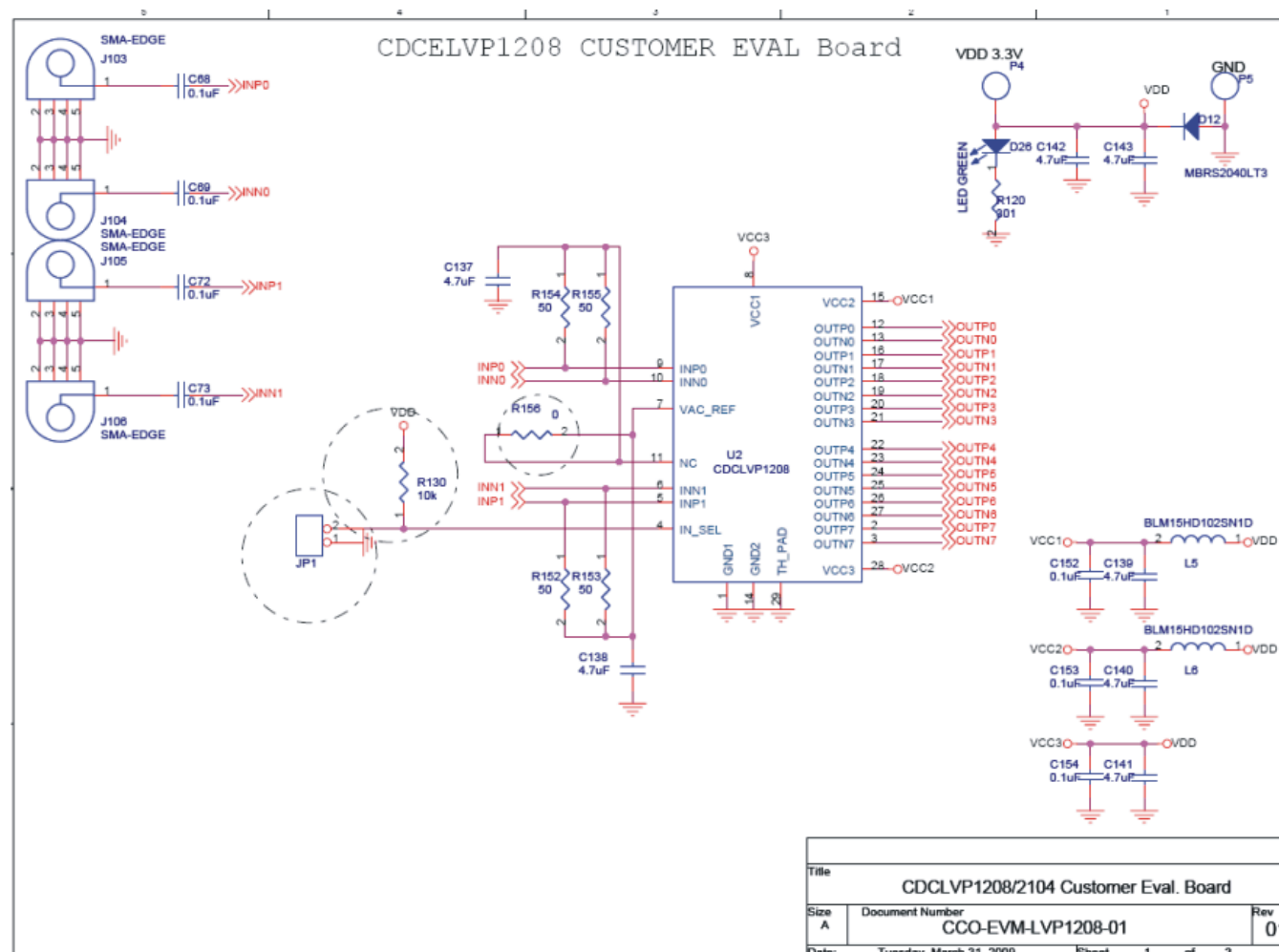
Figure 2. CDCLVP1208EVM—Schematic
