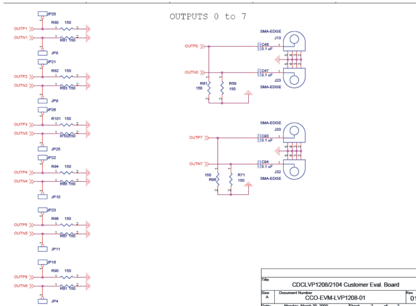
Figure 3. CDCLVP1208EVM—Schematic
