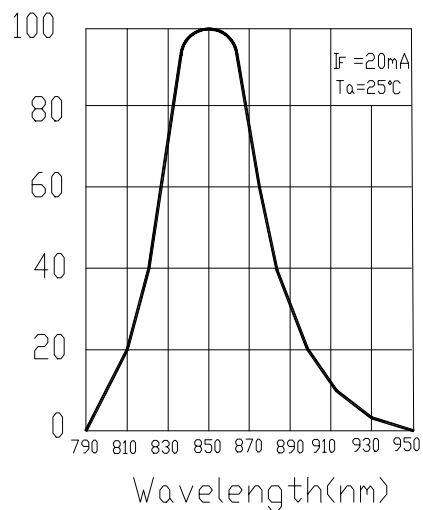
Fig. 2 Spectral Distribution
