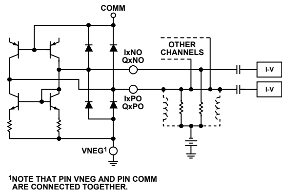
Figure 56. Bypassing the Internal Current Mirrors
