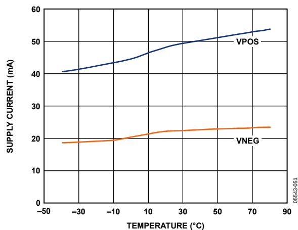
Figure 40. Quiescent Supply Current vs. Temperature
