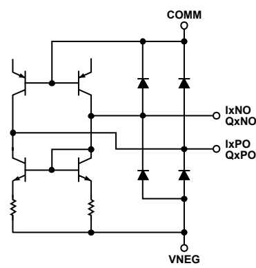
Figure 7. Output Drivers
