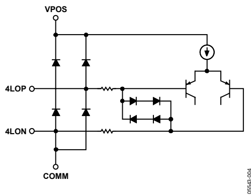
Figure 4. Local Oscillator Inputs
