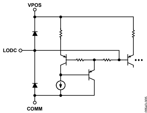
Figure 5. LO Decoupling Pin
