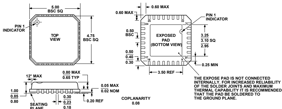
Figure 63. 32-Lead Lead Frame Chip Scale Package [LFCSP_VQ] 5 mm x 5 mm Body, Very Thin Quad (CP-32-2) Dimensions shown in millimeters
