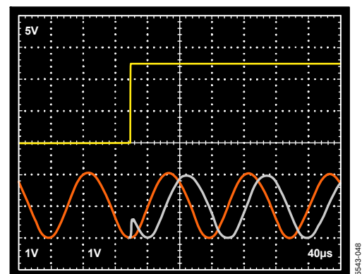
Figure 37. Phase Shifting Response—CH2 Leads CH1 by 90° Top: Input to PH21, Select Code = 0100 Red: Ref CH1 IOUT, Gray: CH2 IOUT Phase Shifted 90° CH1 Ref Phase Code = 0000
