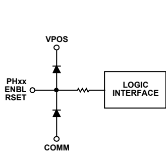
Figure 3. Logic Inputs
