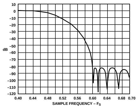
Figure 40. Digital-to-Analog Frequency Response—Transition Band (Full-Scale Inputs, 0 dB)
