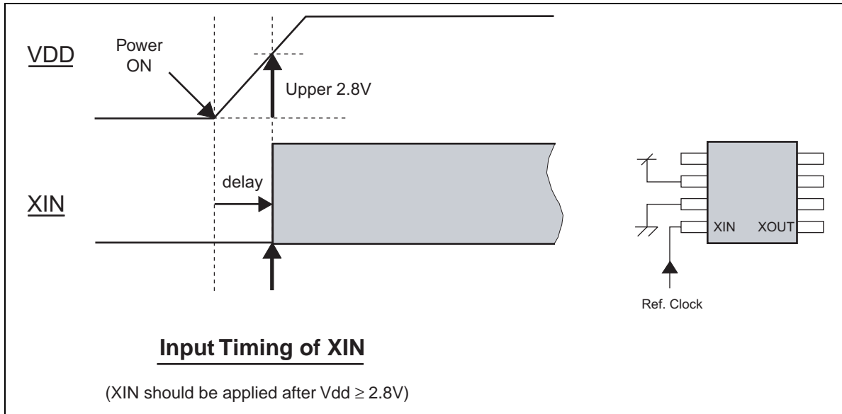
Fig 6-1 In case of reference clock input
