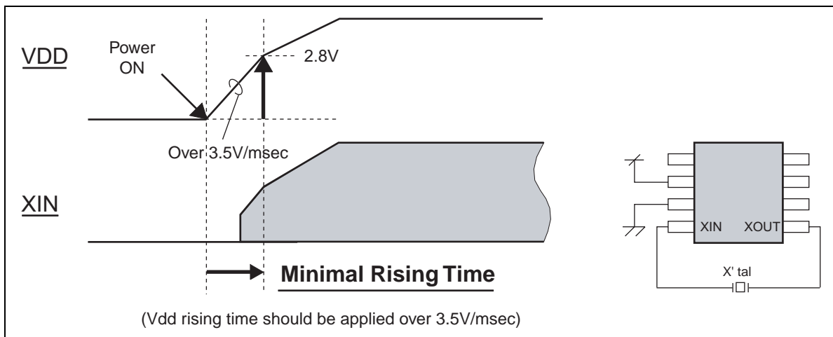
Fig 6-2 In case of X'tal reference input
