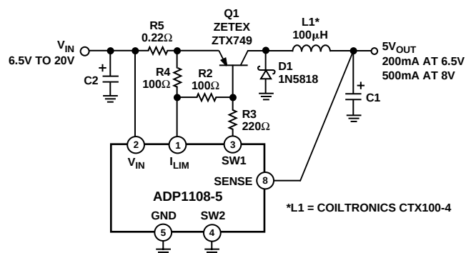
Figure 18. High Current Step-Down Operation
