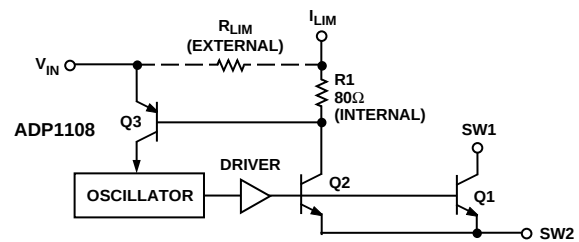
Figure 23. ADP1108 Current Limit Operation
