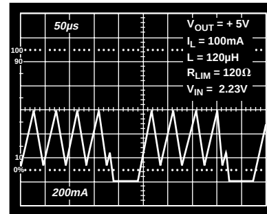
Figure 22. ( I_{LIM} Operation, R_{LIM} = 120 \Omega )
