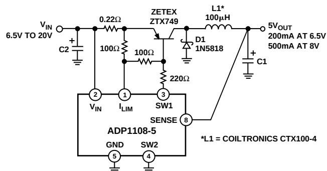
Figure 25. 6.5 V to 5 V Step-Down Converter
