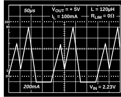
Figure 21. ( I_{LIM} Operation, R_{LIM} = 0 \Omega )
