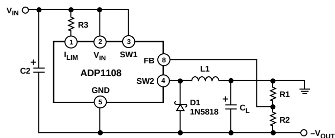
Figure 19. A Positive-to-Negative Converter
