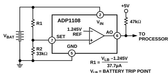
Figure 24a. Setting the Low Battery Detector Trip Point
