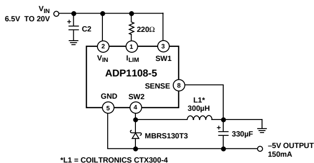
Figure 26. Positive to -5 V Converter
