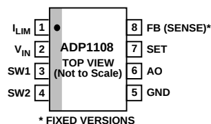
8-Lead SOIC (SO-8)
