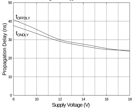
Fig. 17 Propagation Delay vs. Supply Voltage C_L = 15\text{nF} V_{IN} = 5\text{V@1kHz}
