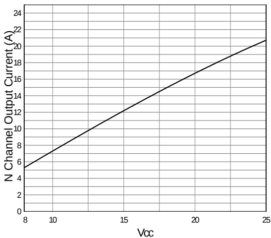
Fig. 27 Vcc vs. N Channel Output Current C L =1uF V IN =0-5V@1kHz
