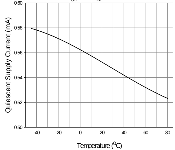
Fig. 20 Quiescent Supply Current vs. Case Temperature V_{CC} = 18\text{V} V_{IN} = 5\text{V@1kHz}
