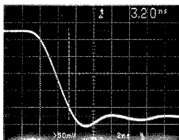
FIGURE 8b. LM1282 Fall Time
