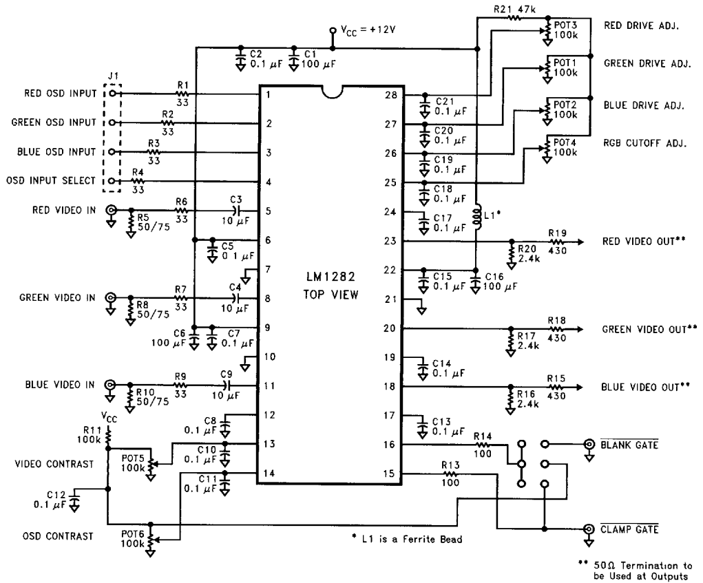
FIGURE 7. LM1282 OSD Video Preamp Demonstration Board Schematic
