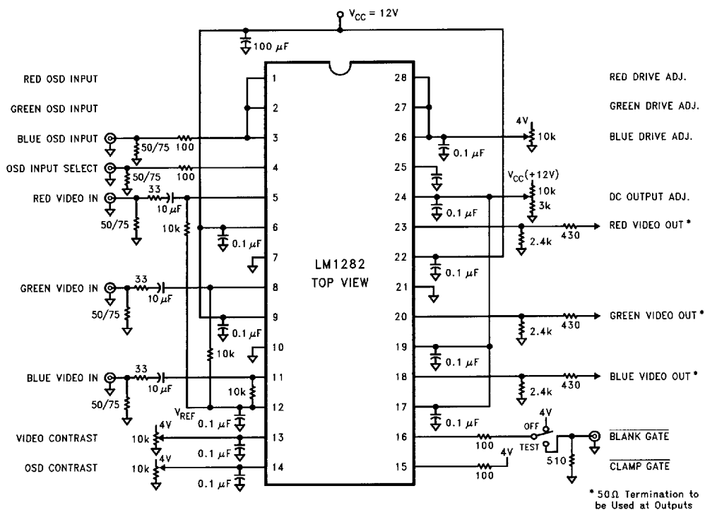
FIGURE 6. LM1282 OSD Video Preamp AC Test Circuit
