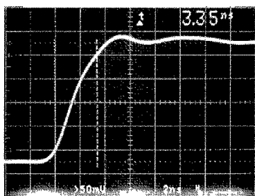
FIGURE 8a. LM1282 Rise Time
