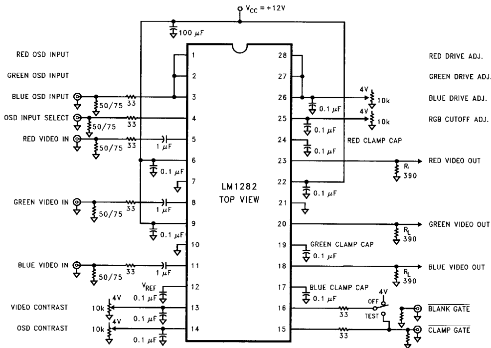
FIGURE 5. LM1282 OSD Video Preamp DC Test Circuit
