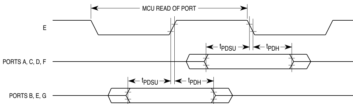
Figure A-7 Port Read Timing Diagram
