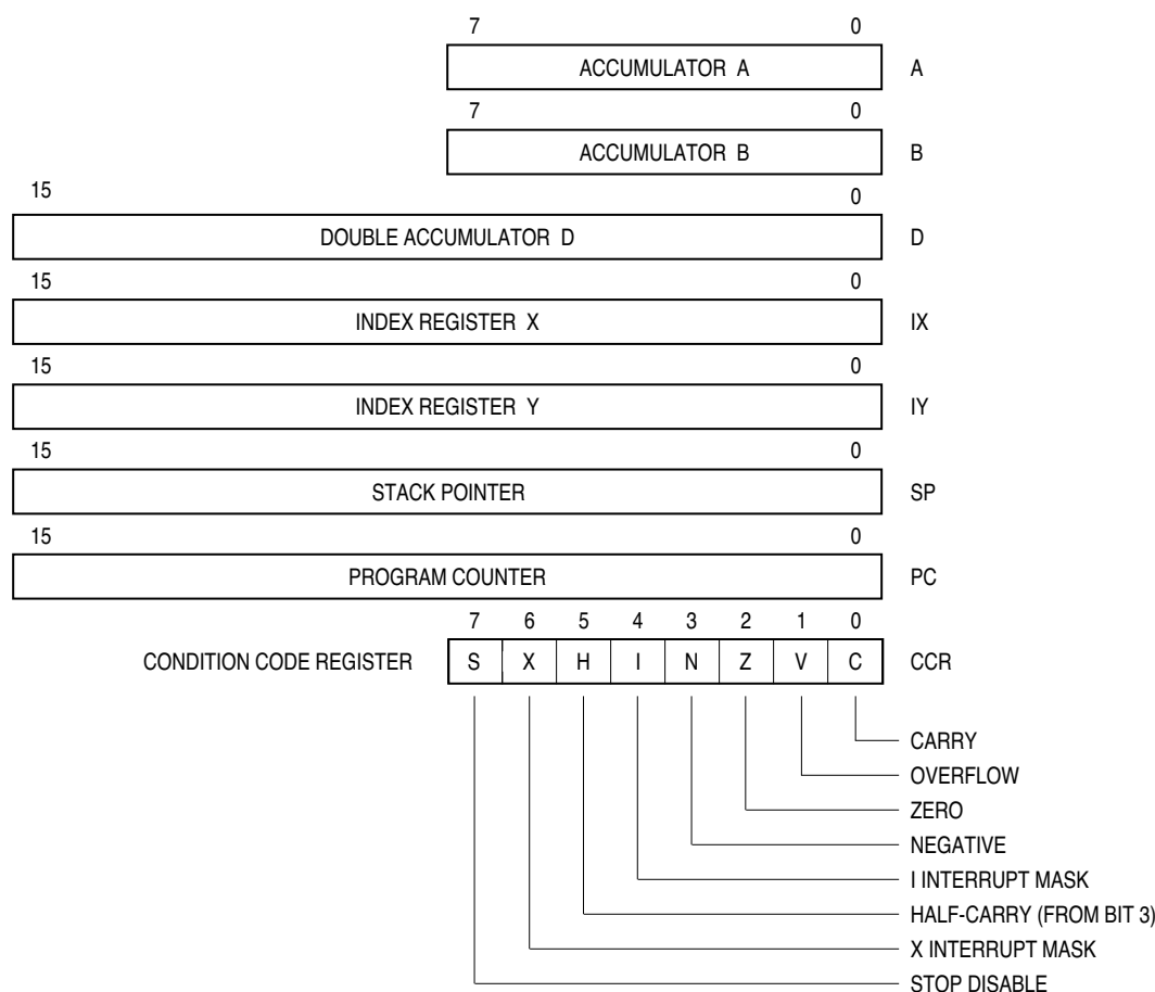
Figure 3-1 Programming Model
