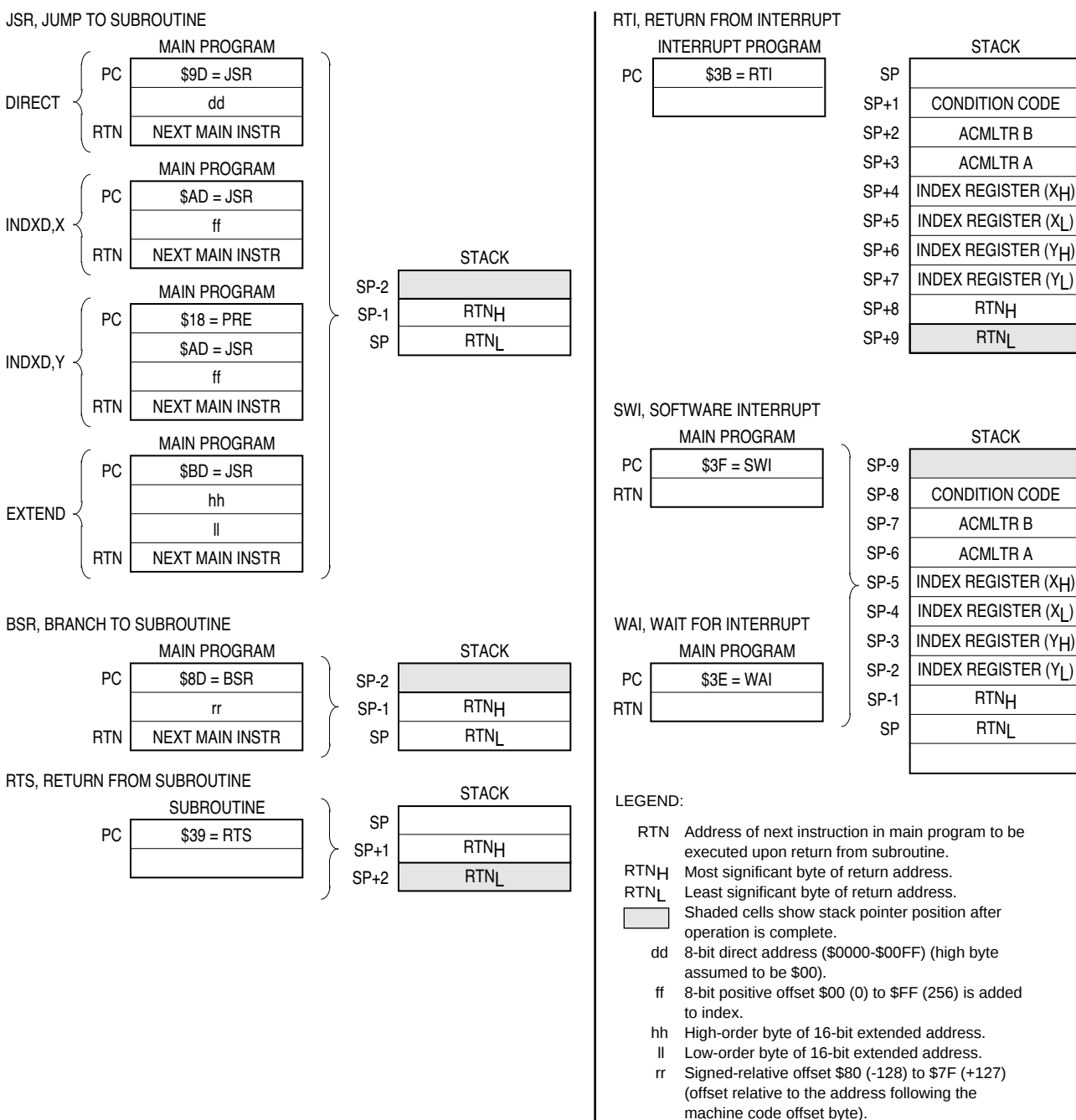
Figure 3-2 Stacking Operations
