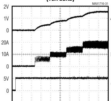
STARTUP WAVEFORM (18A LOAD)
