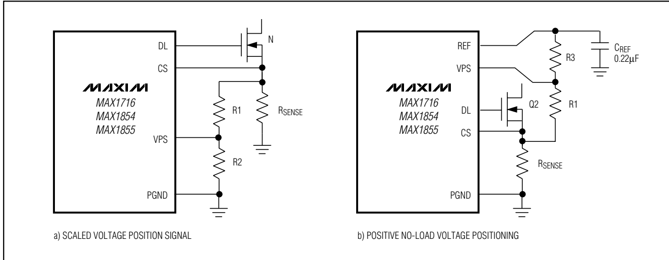
Figure 6. Voltage-Positioning Configurations
