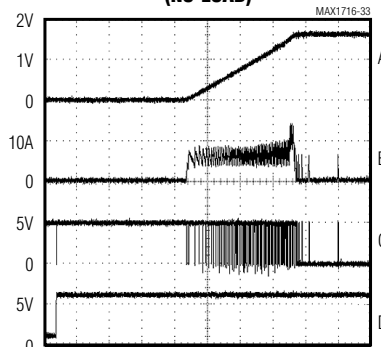
STARTUP WAVEFORM (NO-LOAD)
